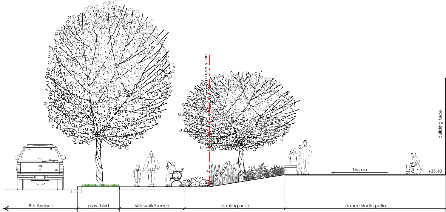
section b - b: 8th Avenue - Dance Studio Patio scale 1:50
