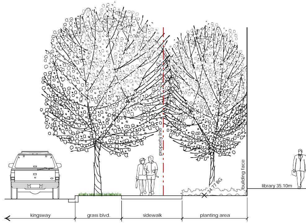
section d - d: kingsway scale 1:50
