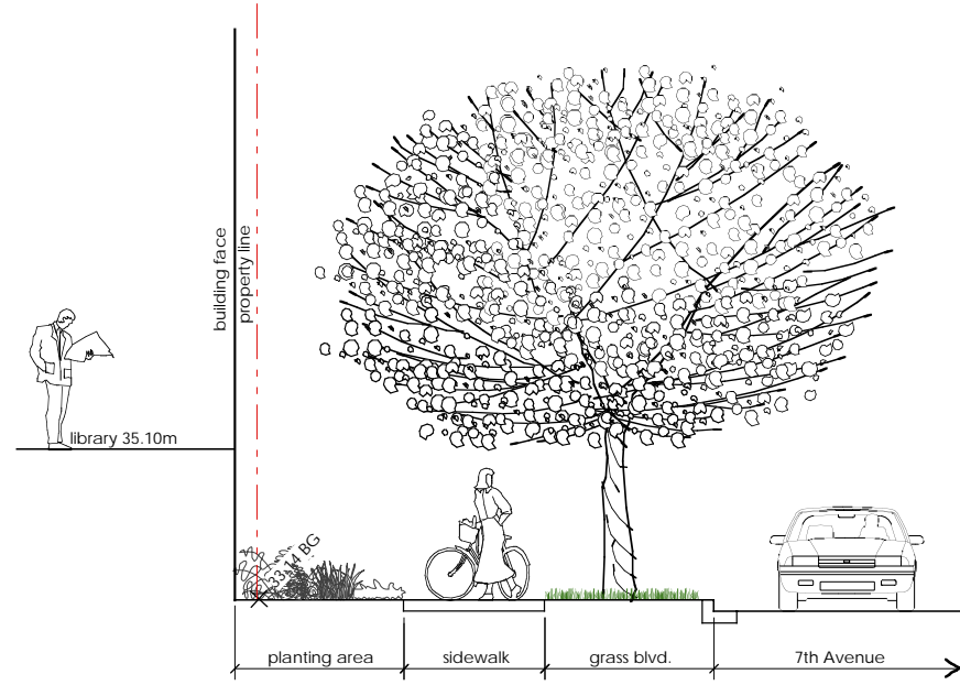
section e - e: 7th Avenue scale 1:50
