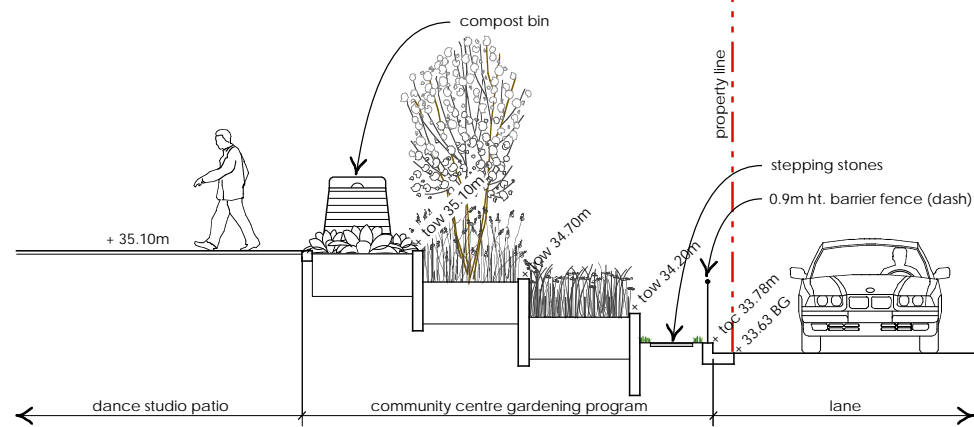
section a - a: dance studio patio - lane scale 1:50
