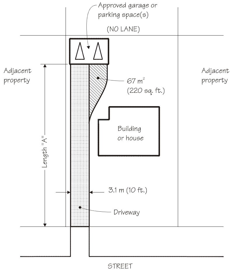
ILLUSTRATIVE PLAN not to scale
