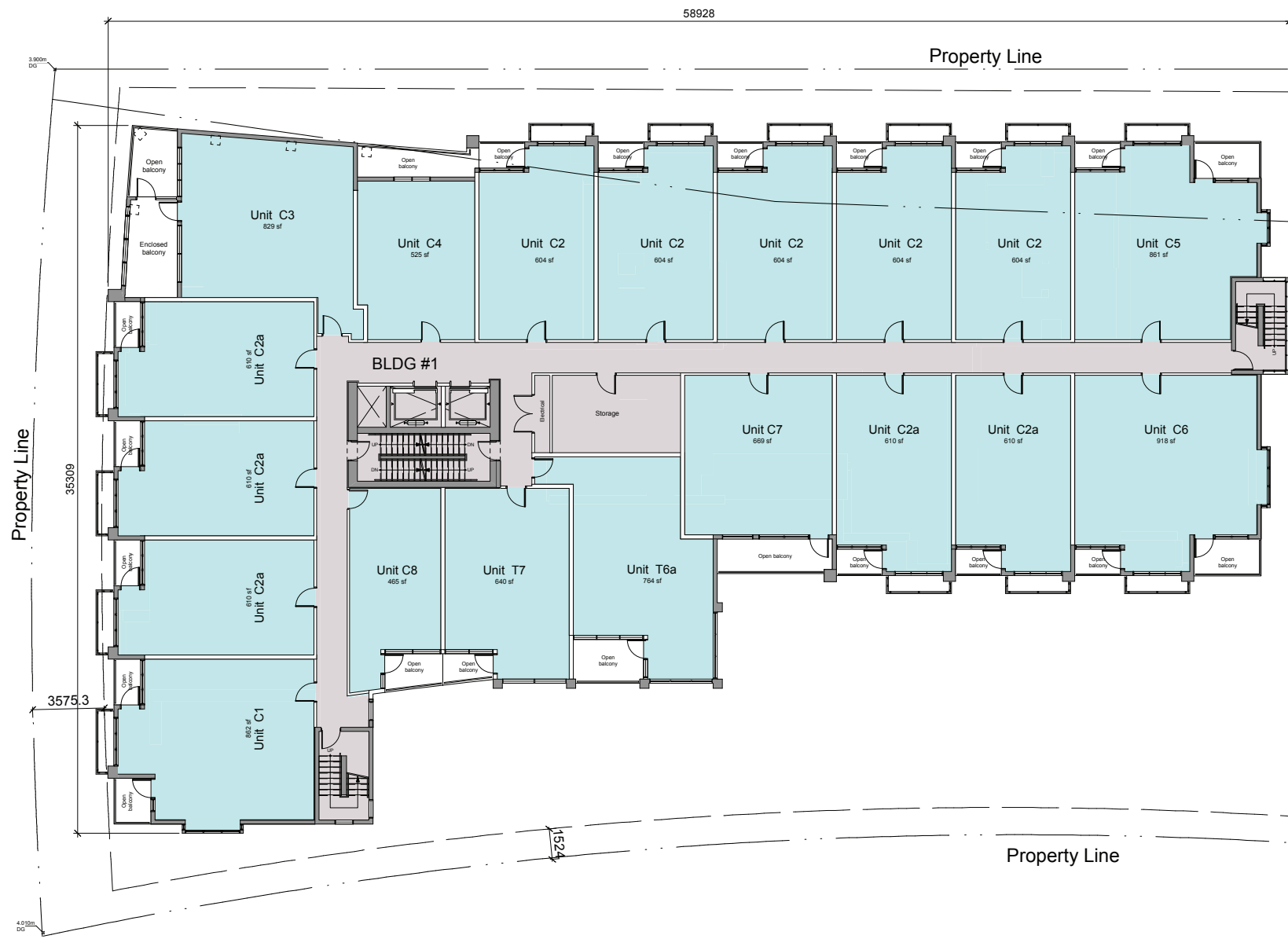
Building 1 Condominium: Level 3 Plan
