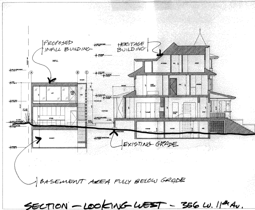
WEST ELEVATION - 356 W. 11TH AVE EXISTING HERITAGE BUILDING WITH PROPOSED ADDITION
