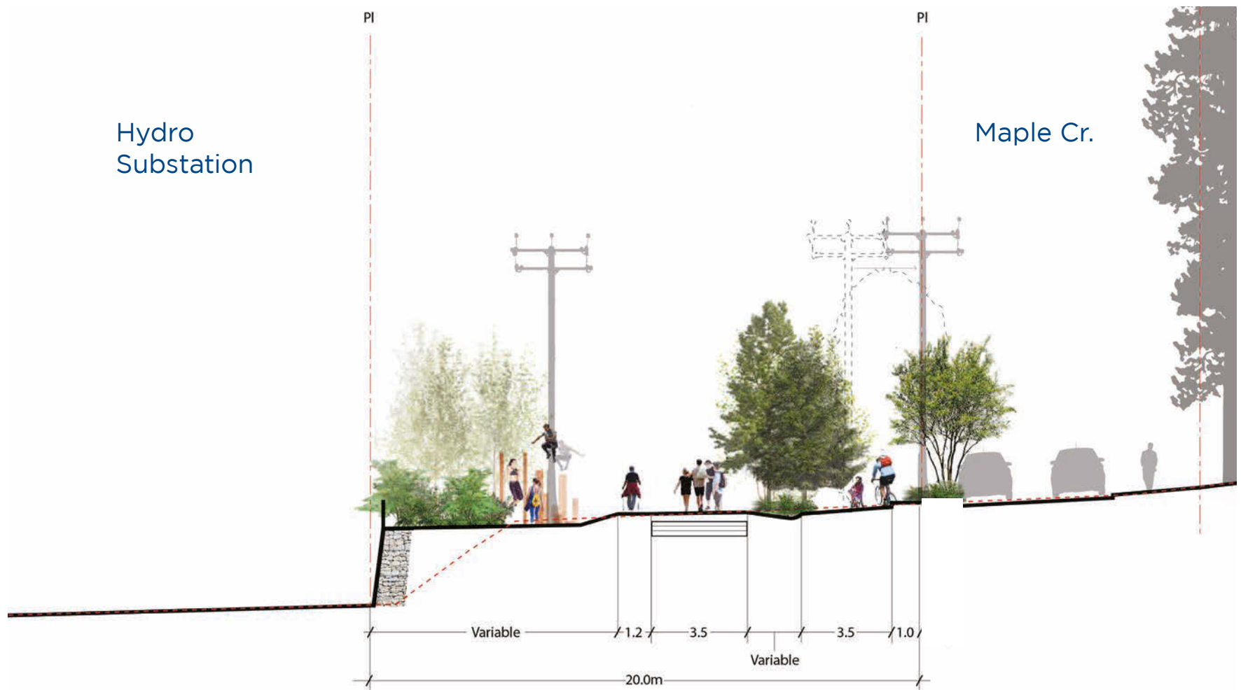
PRE-STREETCAR SECTION - Looking North
