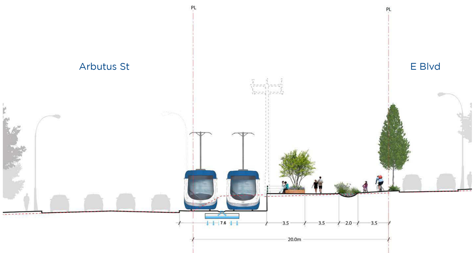
POST-STREETCAR SECTION - Looking North
