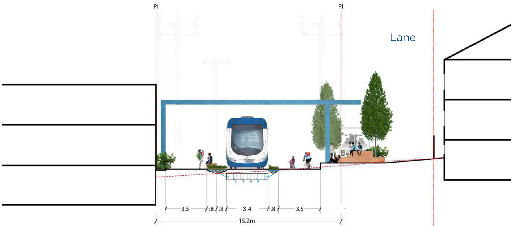
POST-STREETCAR SECTION - Looking North
