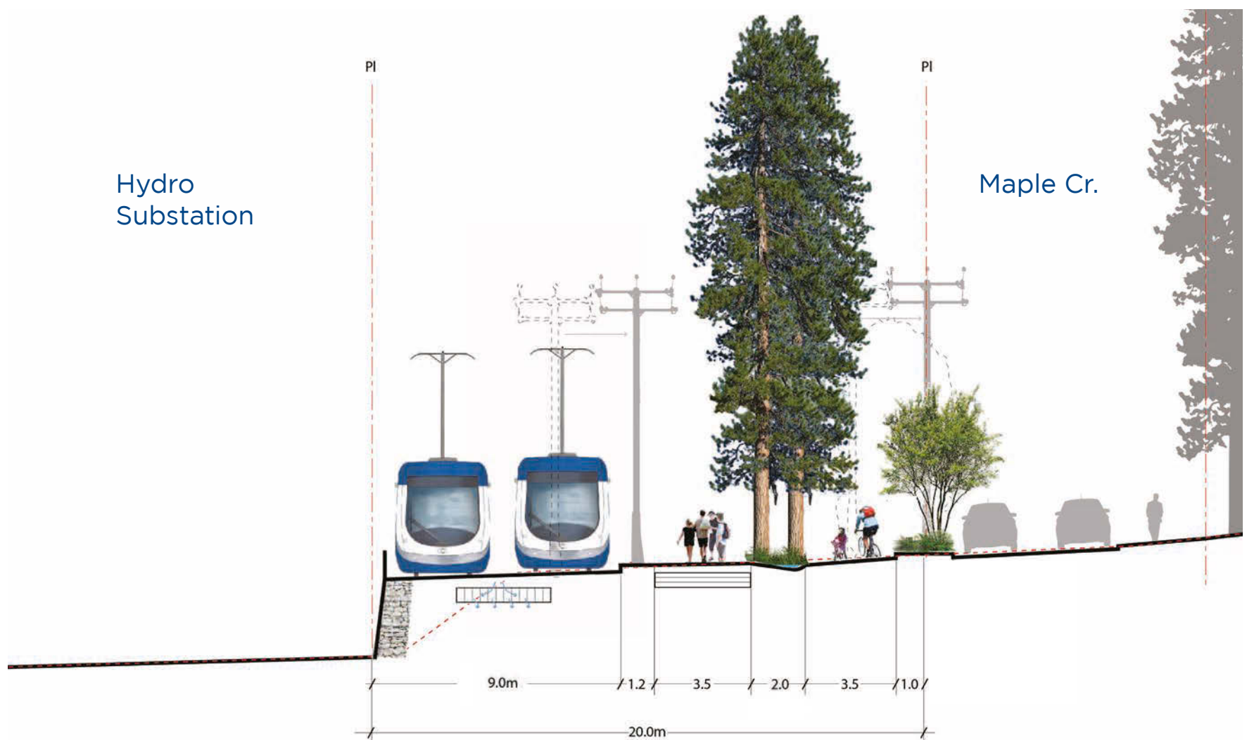
POST-STREETCAR SECTION - Looking North
