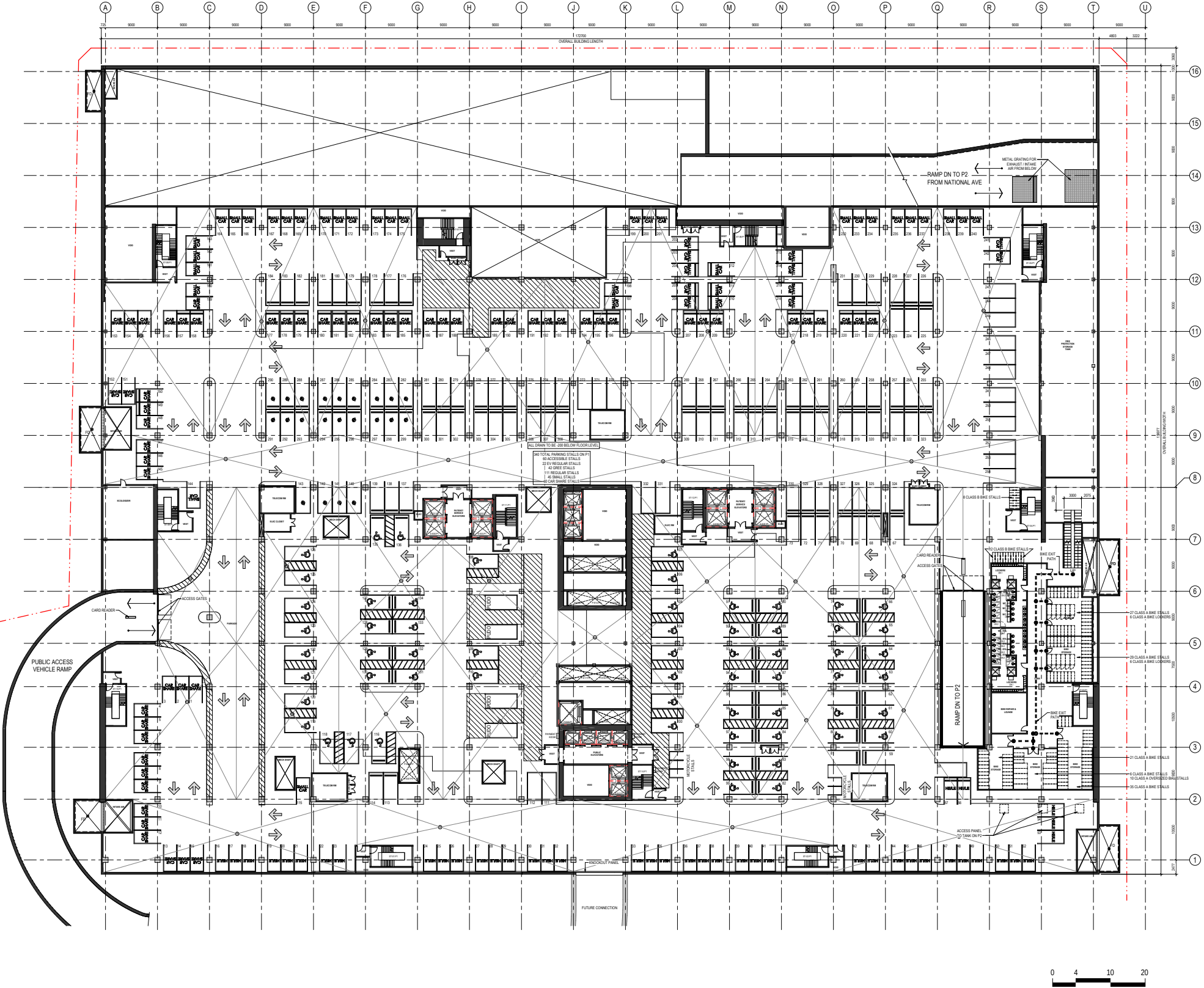
Parking Level P1
