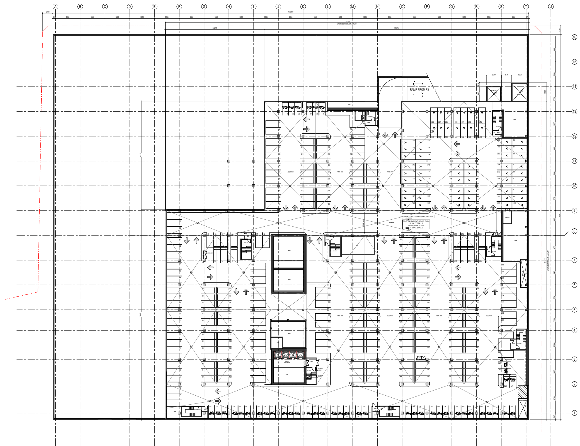
Parking Level P4
