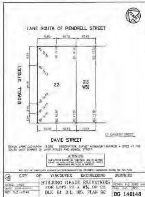
CITY OF VANCOUVER BUILDING GRADE ELEVATIONS SCALE: MTS 2
