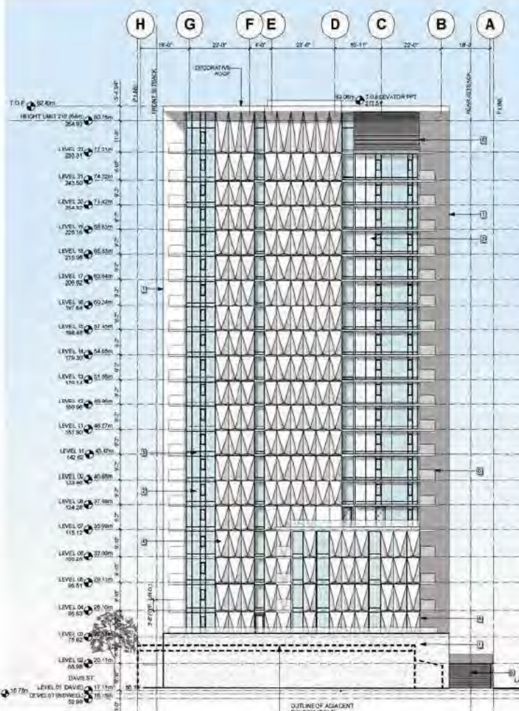
East Elevation Scale: 1/16" = 1'-0" 1
