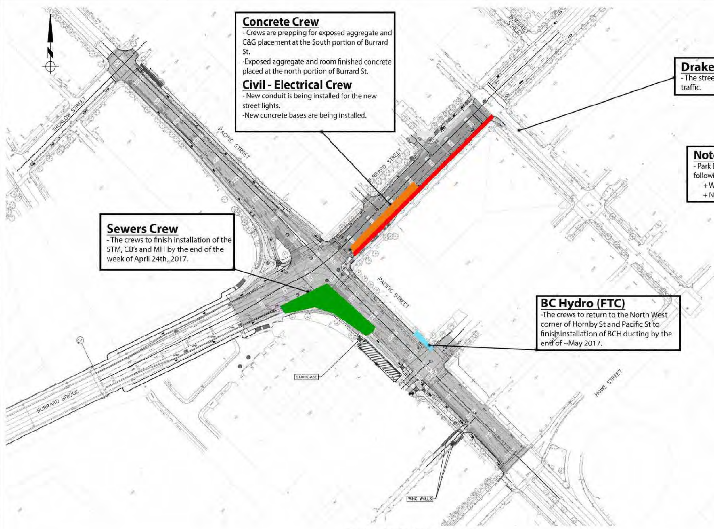
PLAN – SCOPE OF MAJOR WORKS SCALE: 1:750
