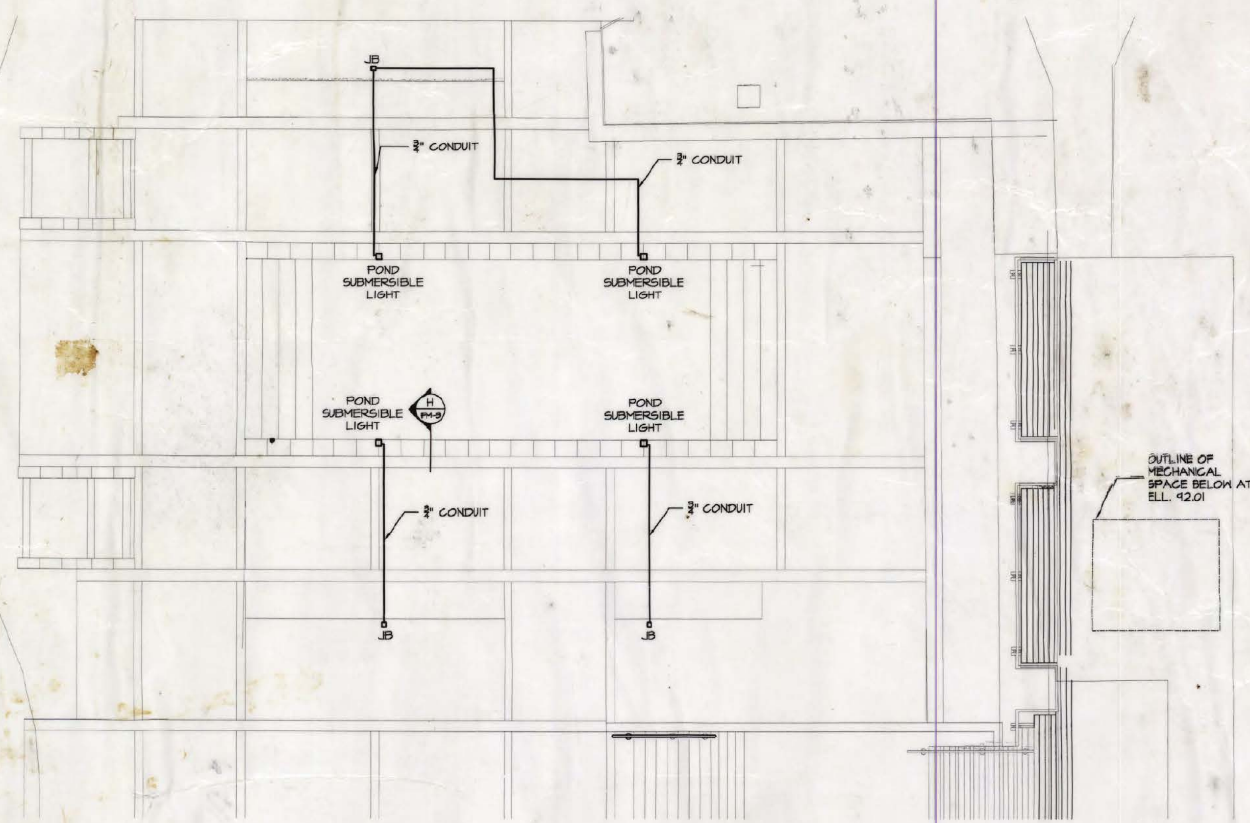
3 LIGHTING PLAN SCALE: 1:100
