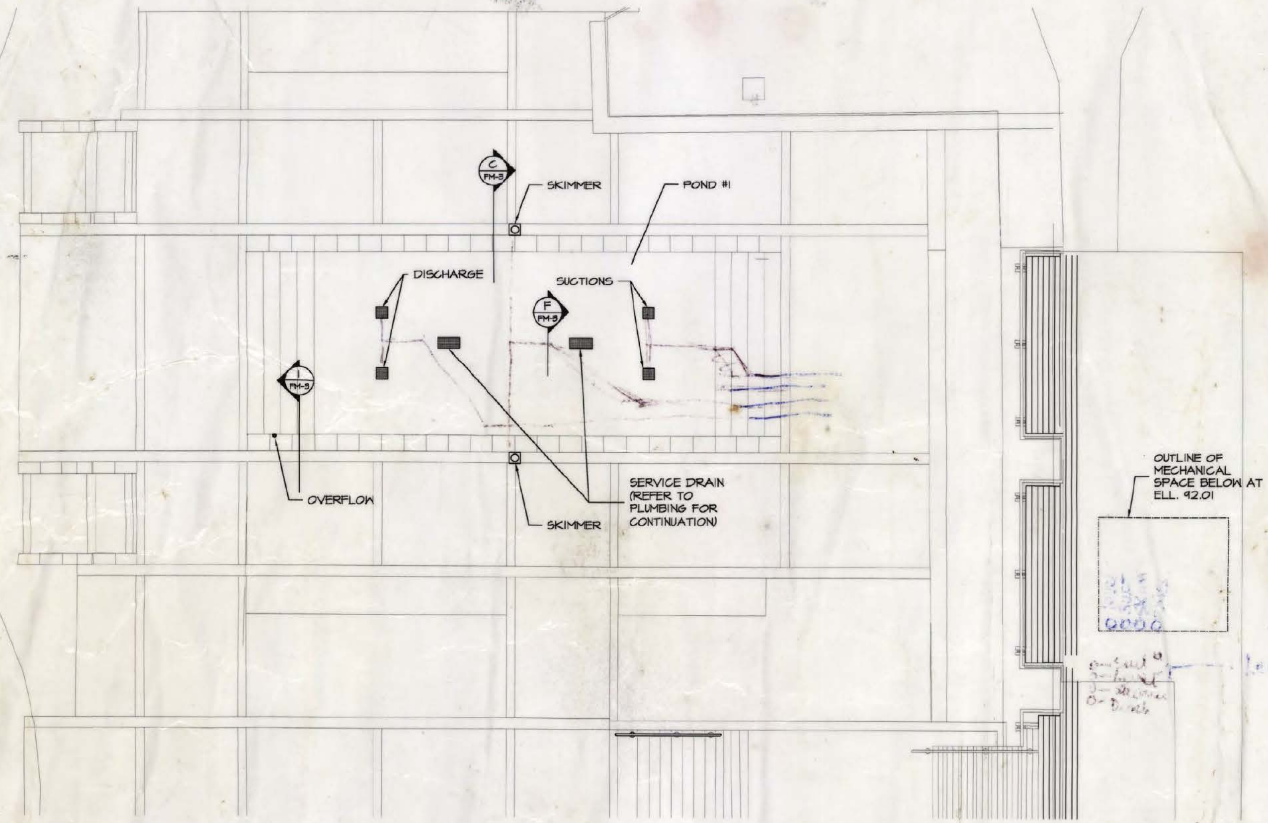
1 FIXTURE PLAN SCALE: 1:100
