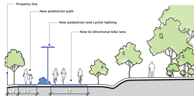
Cross Section C - C' Planned Improvements
