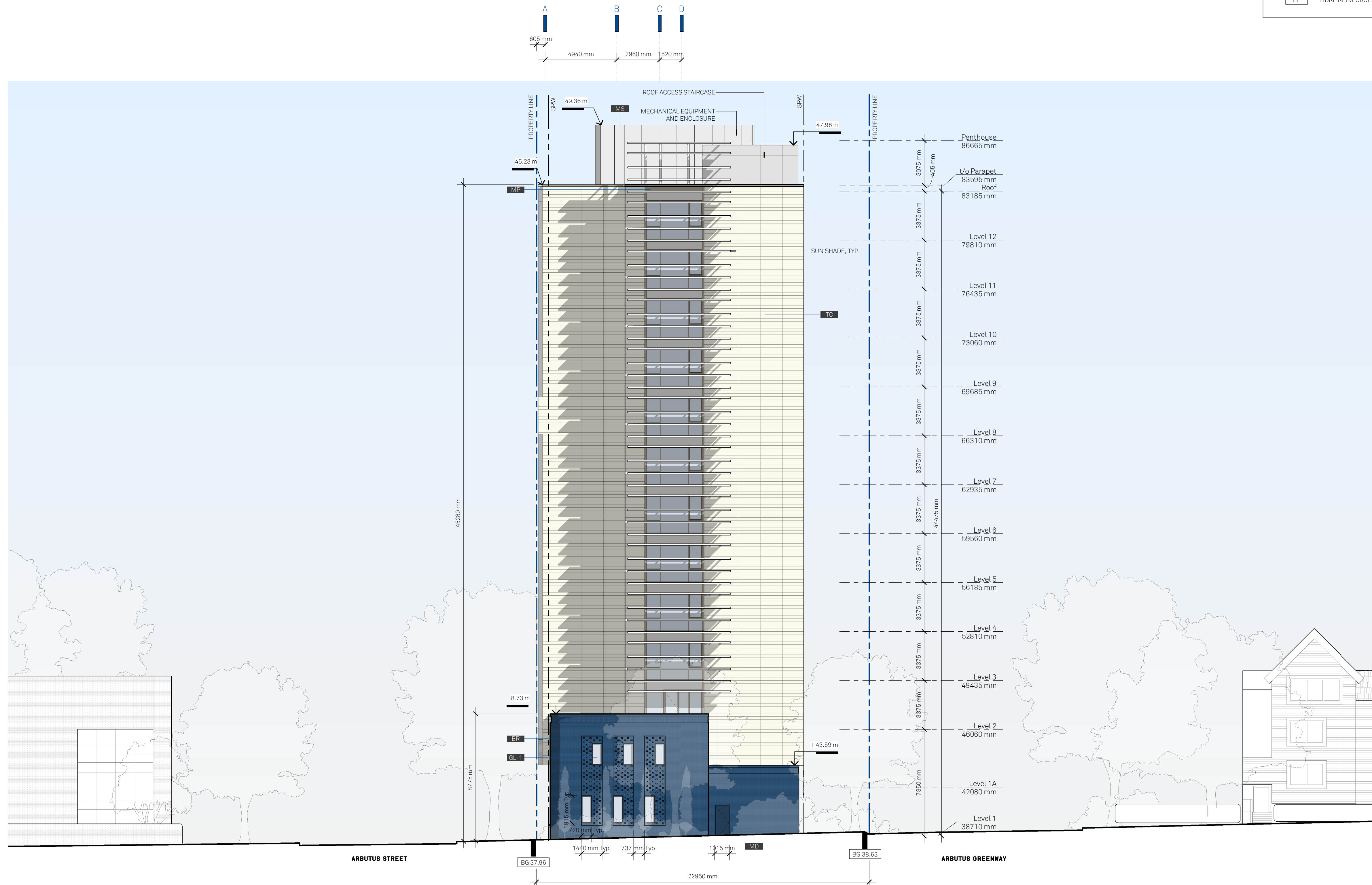
South Elevation
