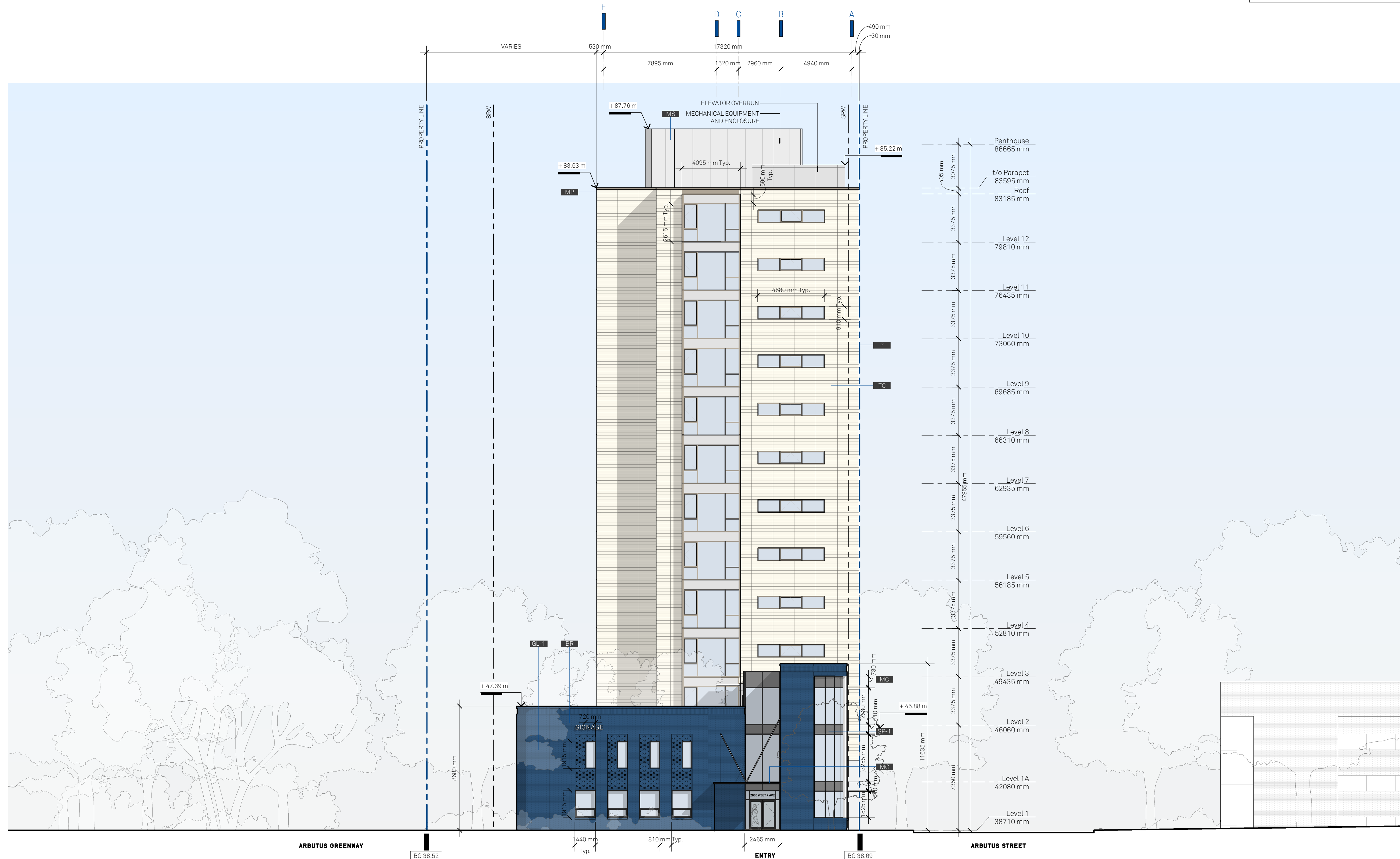
North Elevation
