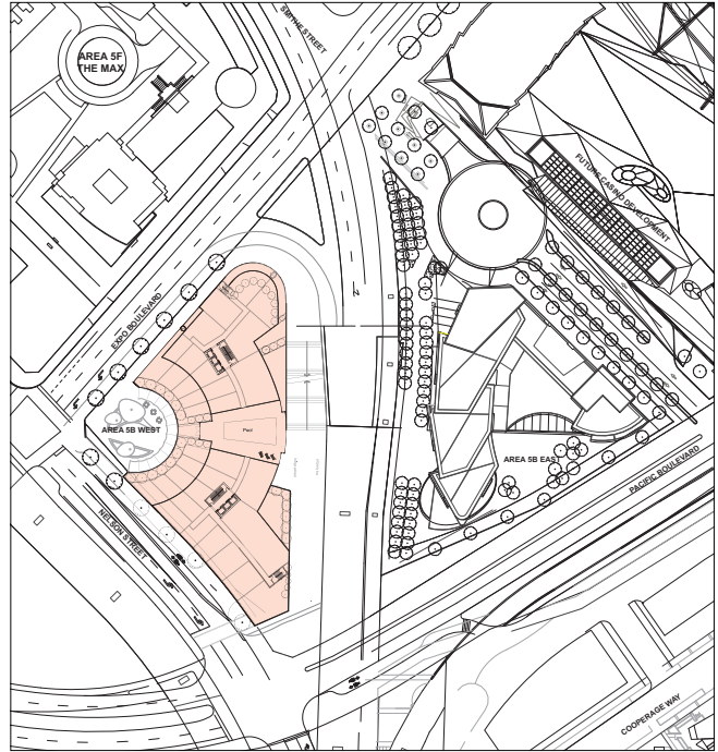
LEVEL 3 PLAN
