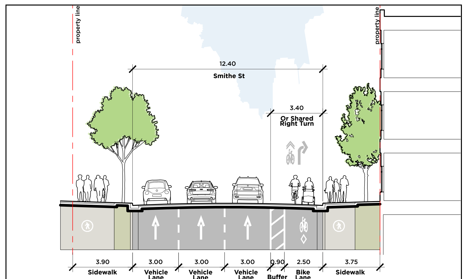
Cross Section: After
