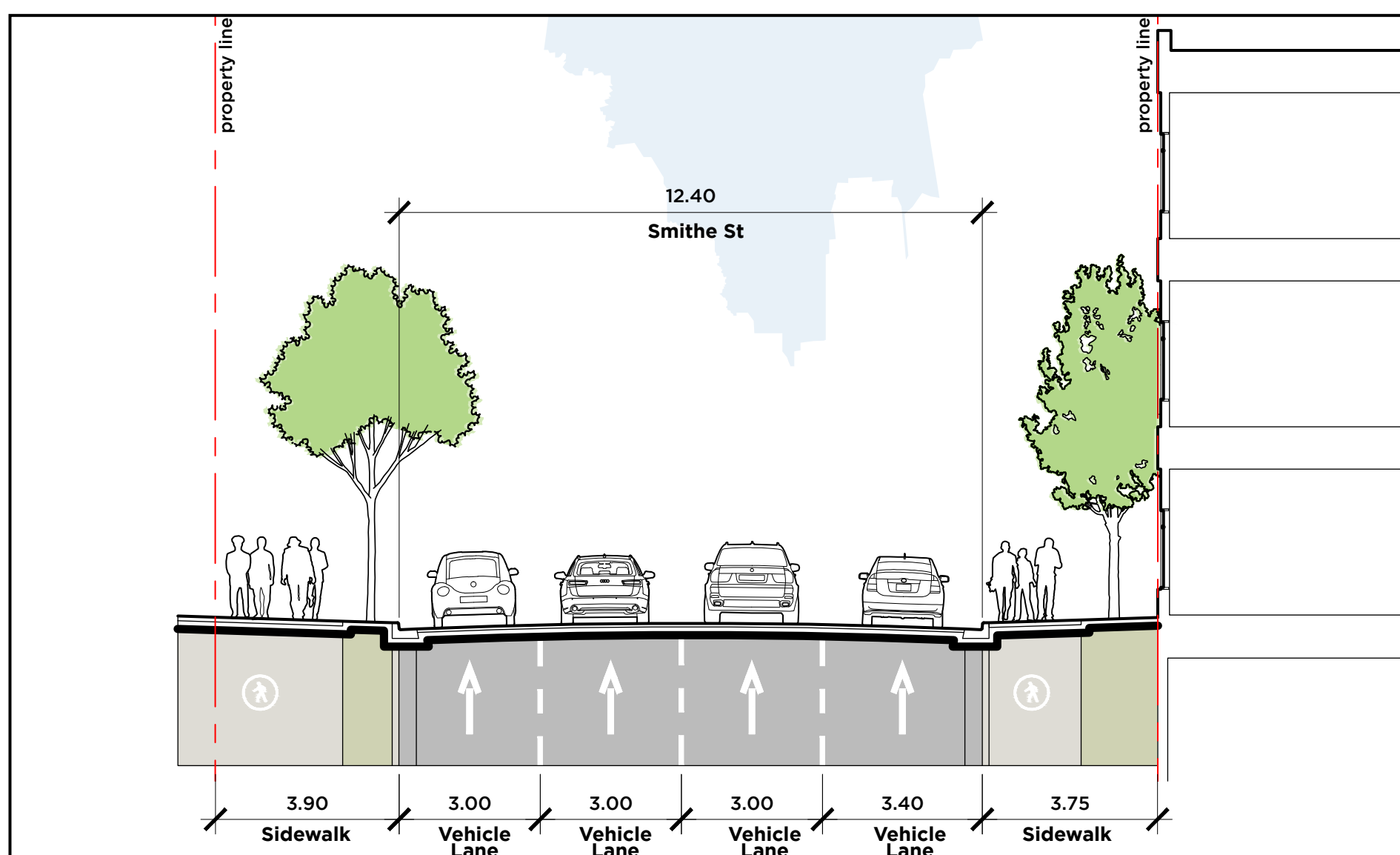
Cross Section: Before
