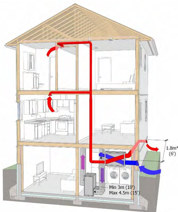
Fig. 2.2 Central HRV as part of furnace system.
