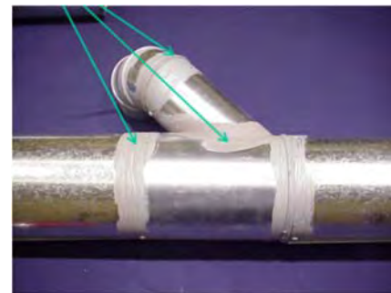
Fig. 4.8 Duct sealing
