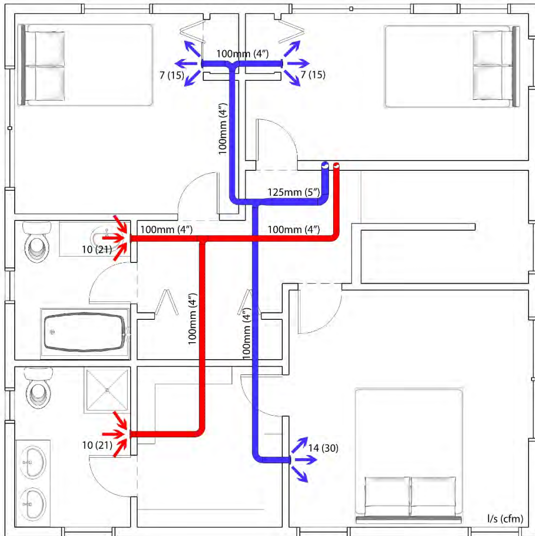
Fig D: Example schematic HRV / ERV trunk & branch ducting system layout, upper floor
