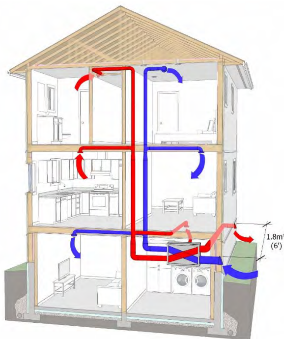
Fig. 2.1 Central HRV system. *Exhaust outlet and supply air inlet separation distance recommended by TECA.
