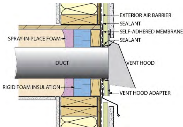
Fig. 4.7 Sample detail of duct penetrating the building's air barrier.
