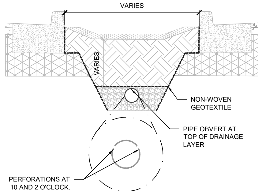
3.7B PARTIALLY INFILTRATING GI UNDERDRAIN
