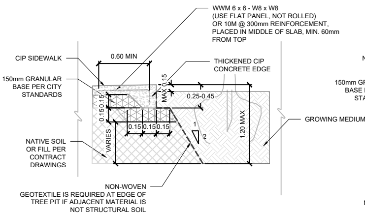
SOIL EXCAVATION, COMPACTION AND BACKFILLING
