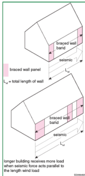
Figure A-9.23.13.7.(4)-A
