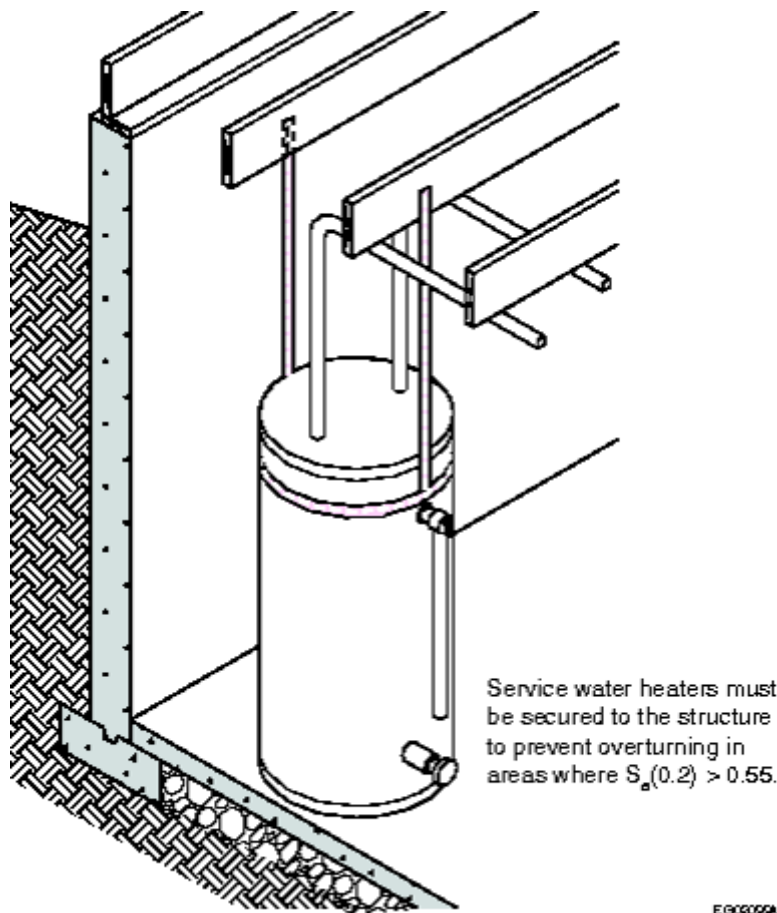
Figure A-9.31.6.2.(3)
