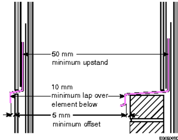
Figure A-9.27.3.8.(4)
