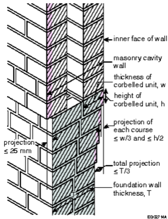
Figure A-9.20.12.2.(2)
