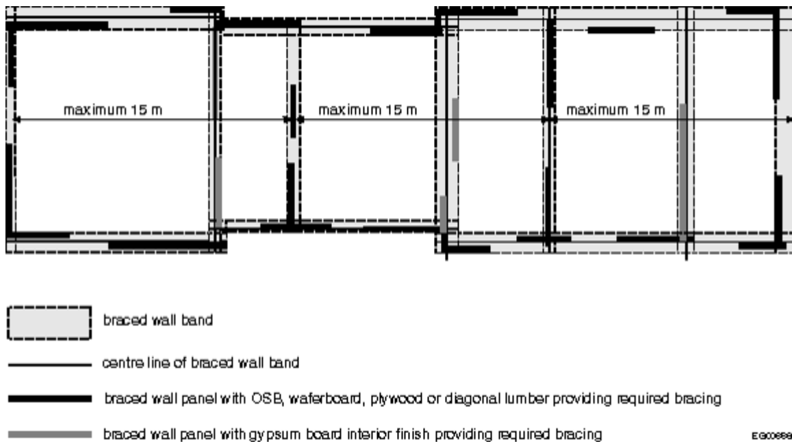
Figure A-9.23.13.6.(3)
