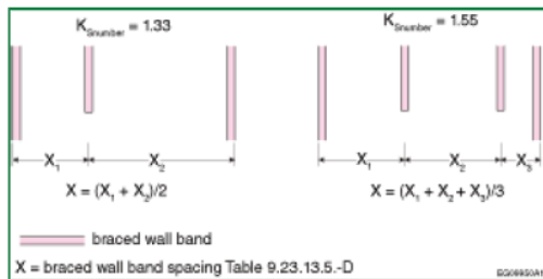
Figure A-9.23.13.7.(4)-C
