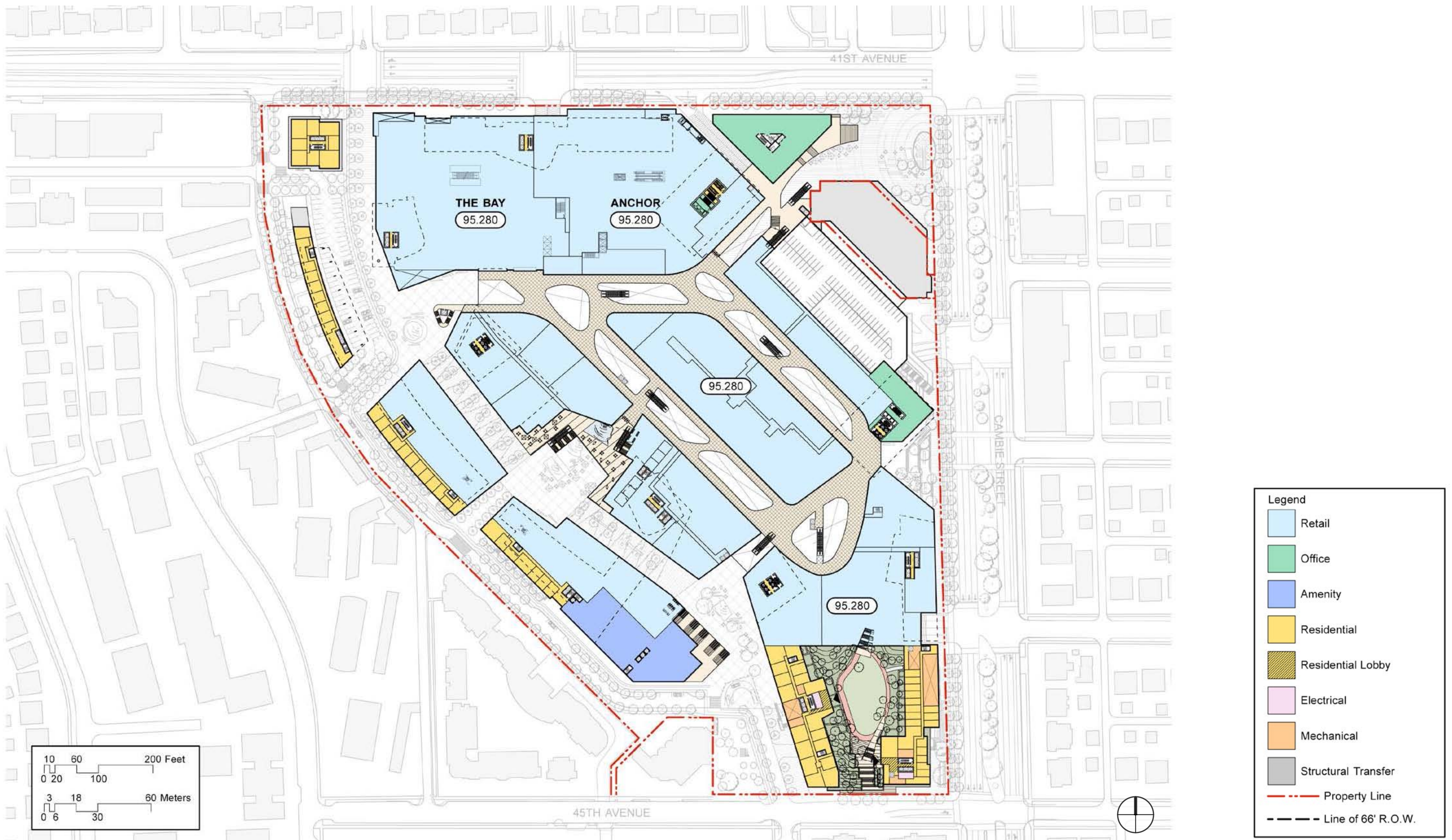
Level 2 Plan
