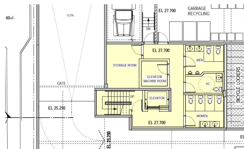
P1 Level 915 F12
