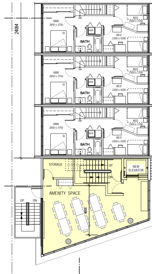
2nd FLOOR 800 ft2
