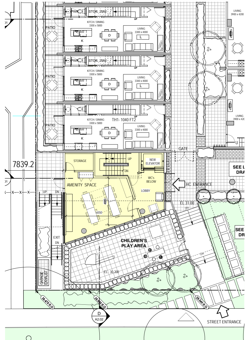
GROUND FLOOR 800 F12
