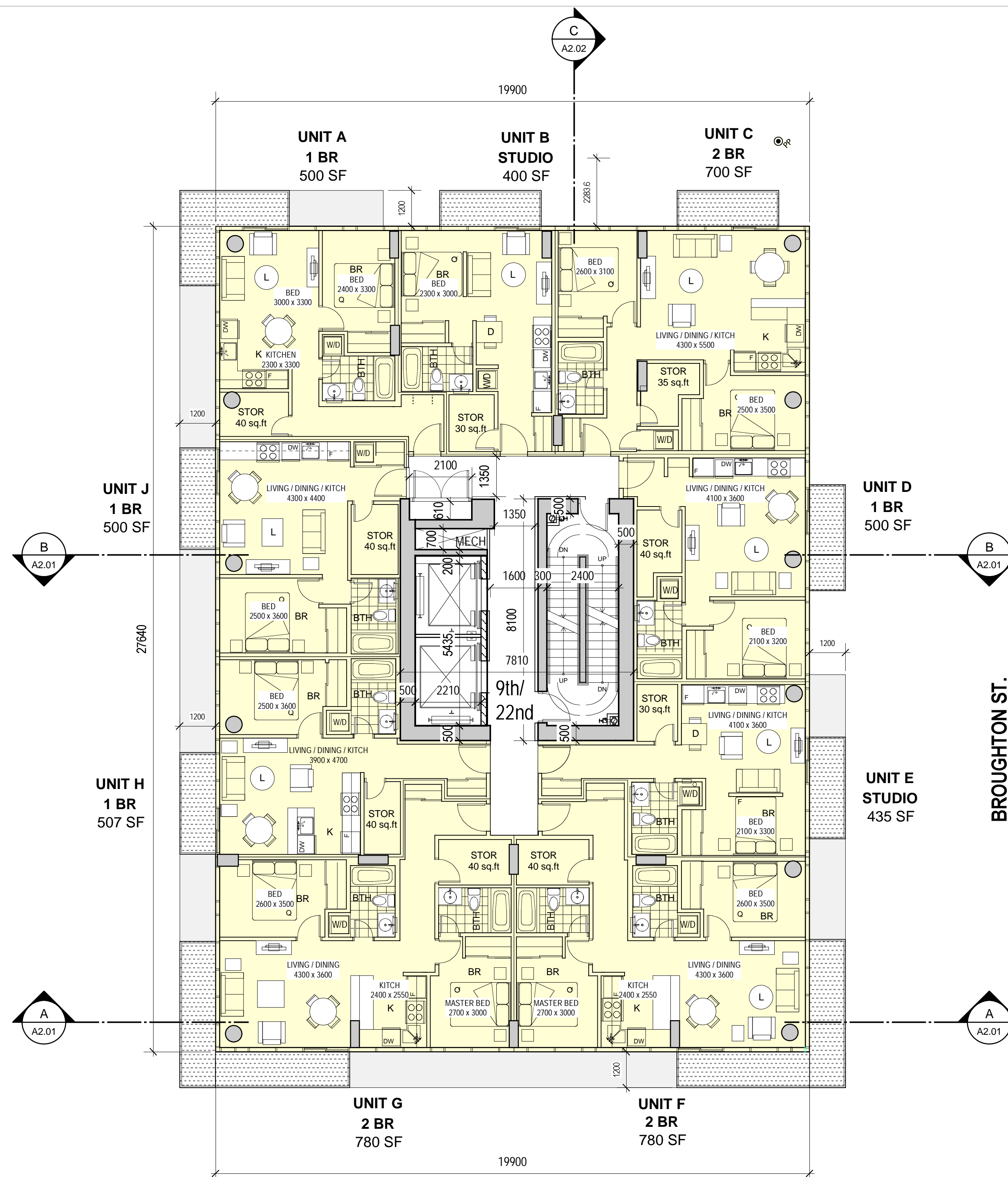
A 9th to 22nd FLOOR PLANS
